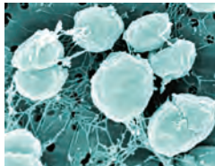
Methane producer, M. jannaschii .
